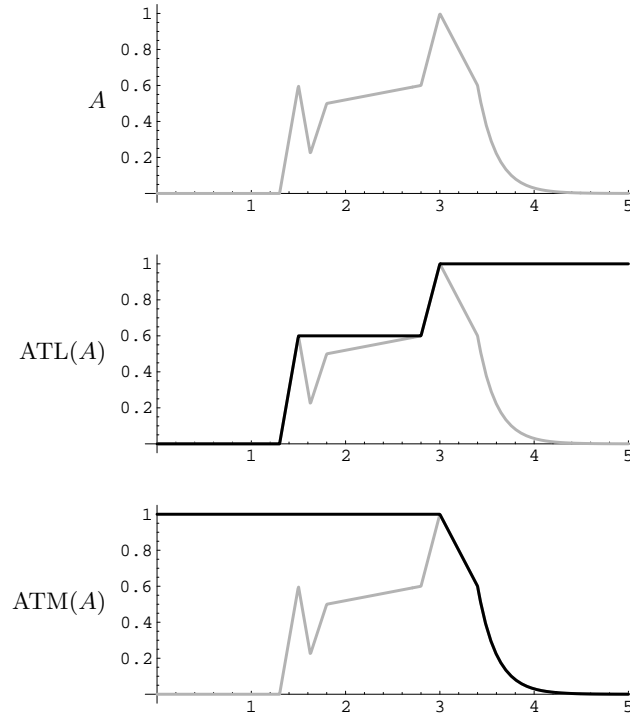
Fig. 3. A fuzzy set A \in \mathcal{F}(\mathbb{R}) and the results which are obtained when applying the operators ATL and ATM
