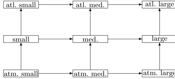
Fig. 1. Hasse diagram of ordering relation \preceq
