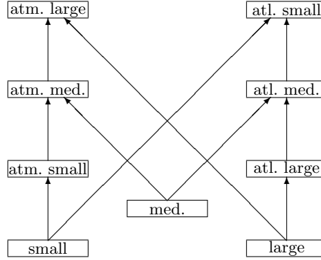
Fig. 2. Hasse diagram of inclusion relation \subseteq
