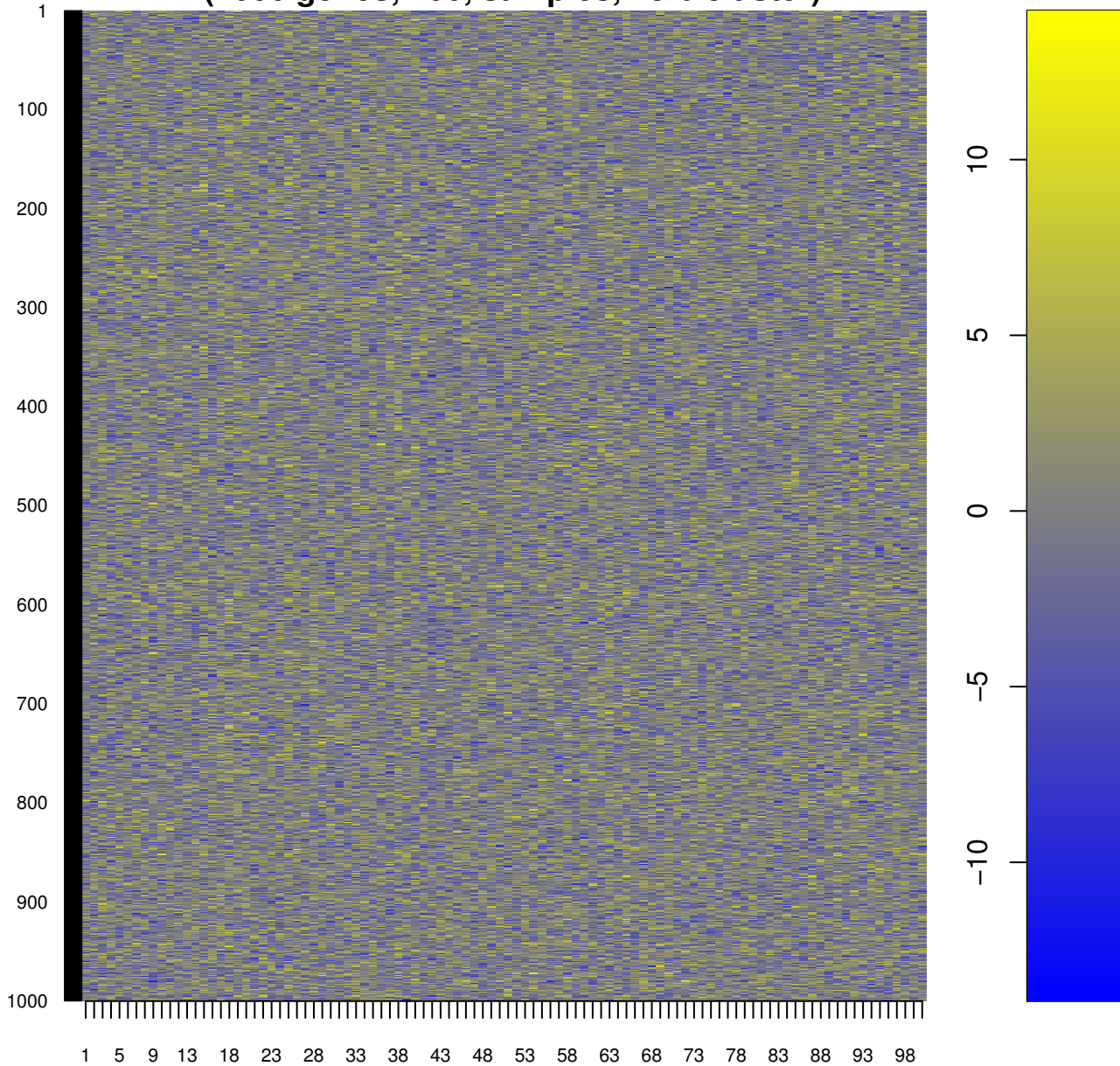
FABIA: data with cluster offset N(0,2) (1000 genes, 100, samples, 13 bicluster)
