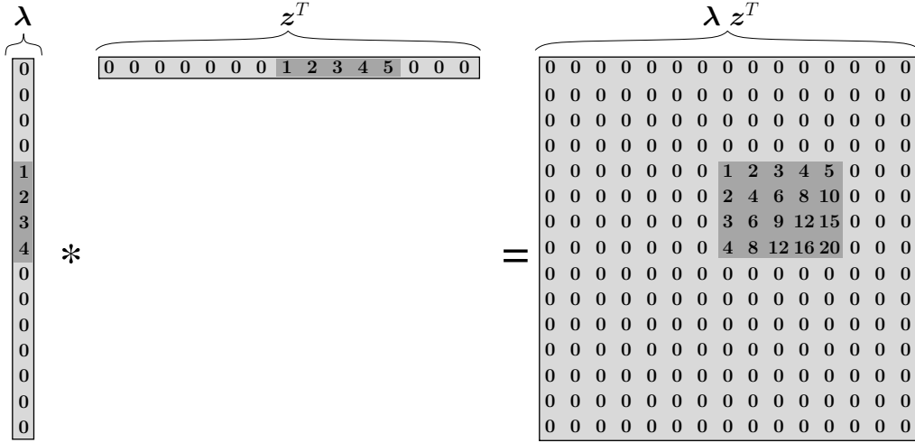
Figure 1: The outer product \lambda z^T of two sparse vectors results in a matrix with a bicluster. Note, that the non-zero entries in the vectors are adjacent to each other for visualization purposes only.
